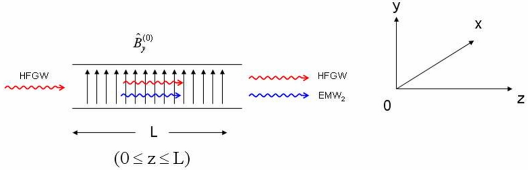
Figure 1: If a HFGW passes through a static magnetic field \hat{B}_y^{(0)} , the interaction of the HFGW with the static magnetic field will produce an EMW, where L is the interacting dimension between the HFGW and the static magnetic field. The EMW 2 has maximum in the terminal position ( Z=L ) of the interacting volume due to the space accumulation effect in the propagating direction the ( z -direction).
