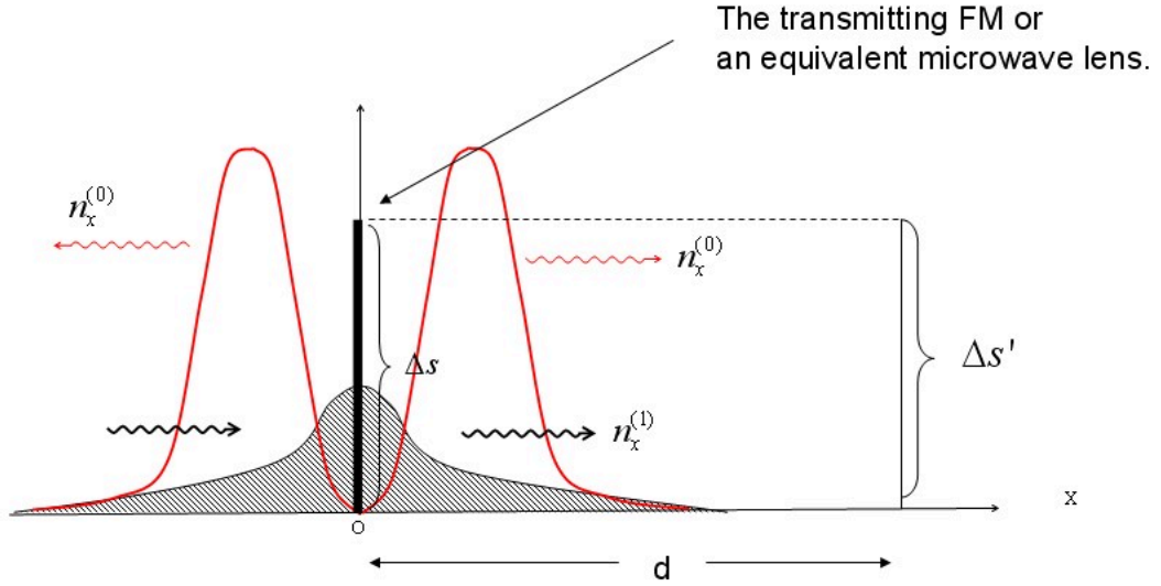
Figure 7: Unlike the photon fluxes N_z^{(0)}, N_z^{(1)}, N_x^{(1)}|_{x=0} = N_x^{(1)}|_{\max} where N_x^{(0)}|_{x=0} = 0 . This means that N_x^{(0)} and N_x^{(1)} focused by the FM at the yz -plane or at the parallel planes very near the yz -plane would have a good focusing effect and the SNR.
