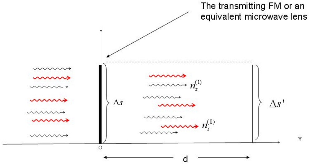
Figure 8: If the FM is just laid at the yz -plane or at the parallel planes very near the yz -plane, then the wave-fronts of the photon fluxes passing through the planes would be the plane or the pseudo-plane, and it is possible to obtain an effective focusing effect.
