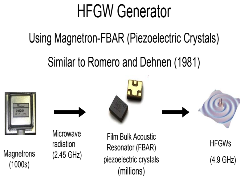
Figure 7. Simplified concept of the HFGW generator.
