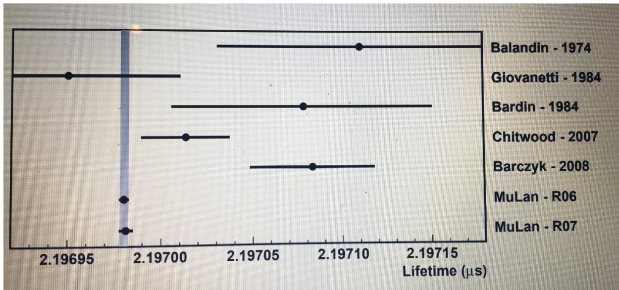
FIG. 2 from D. M. Webber, et al. (2011), the MuLan Collaboration [B5]
