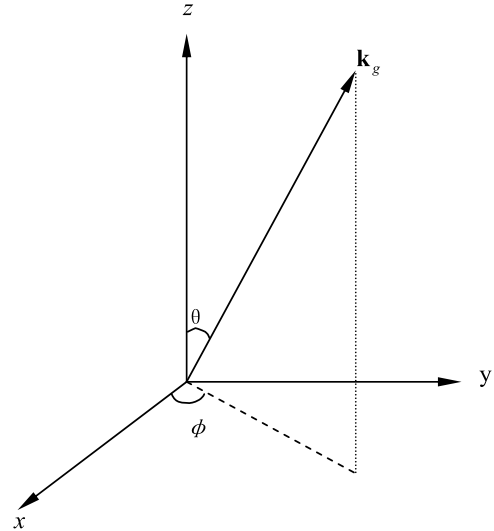
Fig. 8. The z -axis is the symmetrical axis of the Gaussian beam, k_g represents the propagating direction of the arbitrary component of the relic GW
