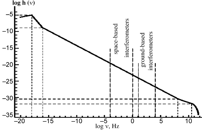
Fig. 7. Envelope of the h_{\text{rms}}(\nu) spectrum for a certain parameter condition. The figure is taken from [41]. The envelope shows that the r.m.s. values of the HFRGW amplitudes in the region of 10^8 – 10^{10} Hz would be \sim 10^{-30} – 10^{-32}/\sqrt{\text{Hz}} , roughly
